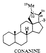
CONANINE
