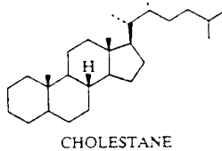
CHOLESTANE
