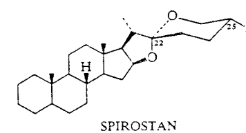
SPIROSTAN
