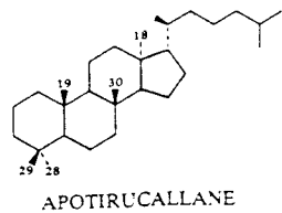
APOTIRUCALLANE
