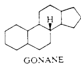
GONANE
