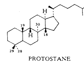
PROTOSTANE
