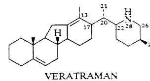
VERATRAMAN
