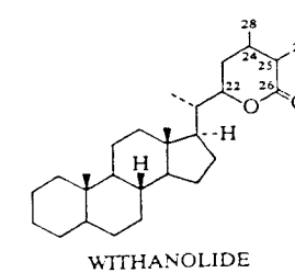
WITHANOLIDE
