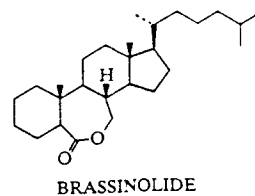
BRASSINOLIDE
