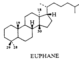
EUPHANE
