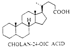
CHOLAN-24-OIC ACID
