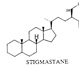
STIGMASTANE
