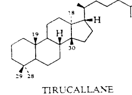
TIRUCALLANE
