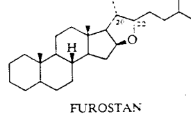
FUROSTAN
