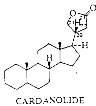
CARDANOLIDE
