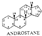
ANDROSTANE
